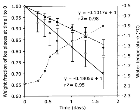
Fig. S3. Evaluation of melting rate of saline ice, with (●) and without (◊) EPS, in a NaCl solution, salinity of 30, that warmed from near freezing at -1.9\text{ }^{\circ}\text{C} to -0.9\text{ }^{\circ}\text{C} (□) over the 1.7-d incubation period. The decrease in ice mass over time was determined for granular ice pieces (initial volume of 100 mL each) formed either from an EPS-free NaCl solution (◊) or the same solution first amended with XG ( 40\text{ mg}\cdot\text{L}^{-1} ; ●) under continuous mechanical stirring to achieve uniform XG and salt content (bulk ice salinity of 8). Floating saline ice pieces, with crushed freshwater ice placed among them to prevent lateral convection, were marked with numbers, weighed at each time point (accuracy of 0.02 g), and returned to position. Data points indicate mean ( n = 5 ) fractional weights of ice at time i relative to time 0; error bars indicate SD of the mean.
